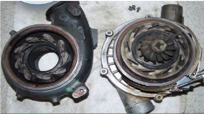
Turbo charger before and after
